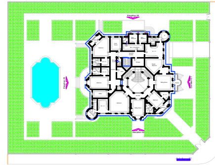
Second Floor Plan A = 508.14 m 2
