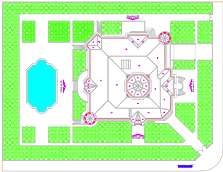
Roof Plan
