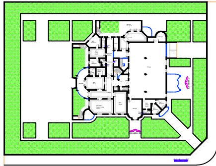
Lower Floor Plan A = 597.77 m 2
